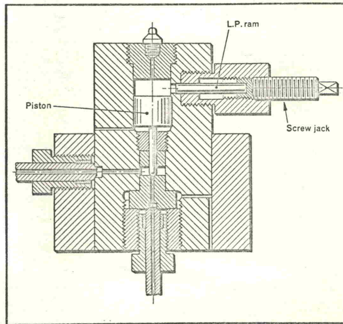
High-pressure valve
